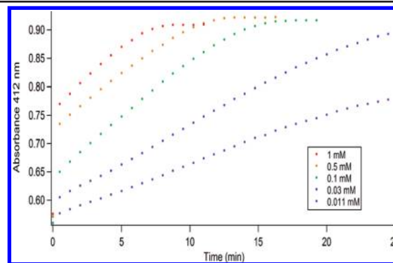
Figure 4. Kinetics traces for the formation of Fe II (TPPS)(NO) at 412 nm from Fe III (TPPS) (9.5 \mu M) and nitrite (10 mM) at different cysteine concentrations (0.011 to 1.0 mM). The time needed to achieve the final spectrum increases with decreasing [CysSH].
