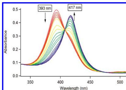
Figure 2. Spectral changes observed as cysteine (0–3 mM) was titrated into a solution of Fe III (TPPS) (5 \mu M) at pH 5.81.
